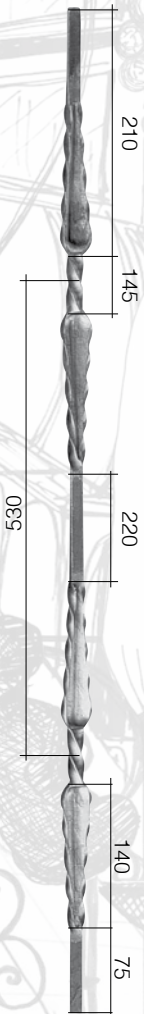
Арт. 1730/1 Φ 12 x 12 mm L 25 mm H 1000 mm
