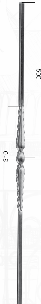
Арт. 1730/7 Φ 12 x 12 mm L 25 mm H 1000 mm
