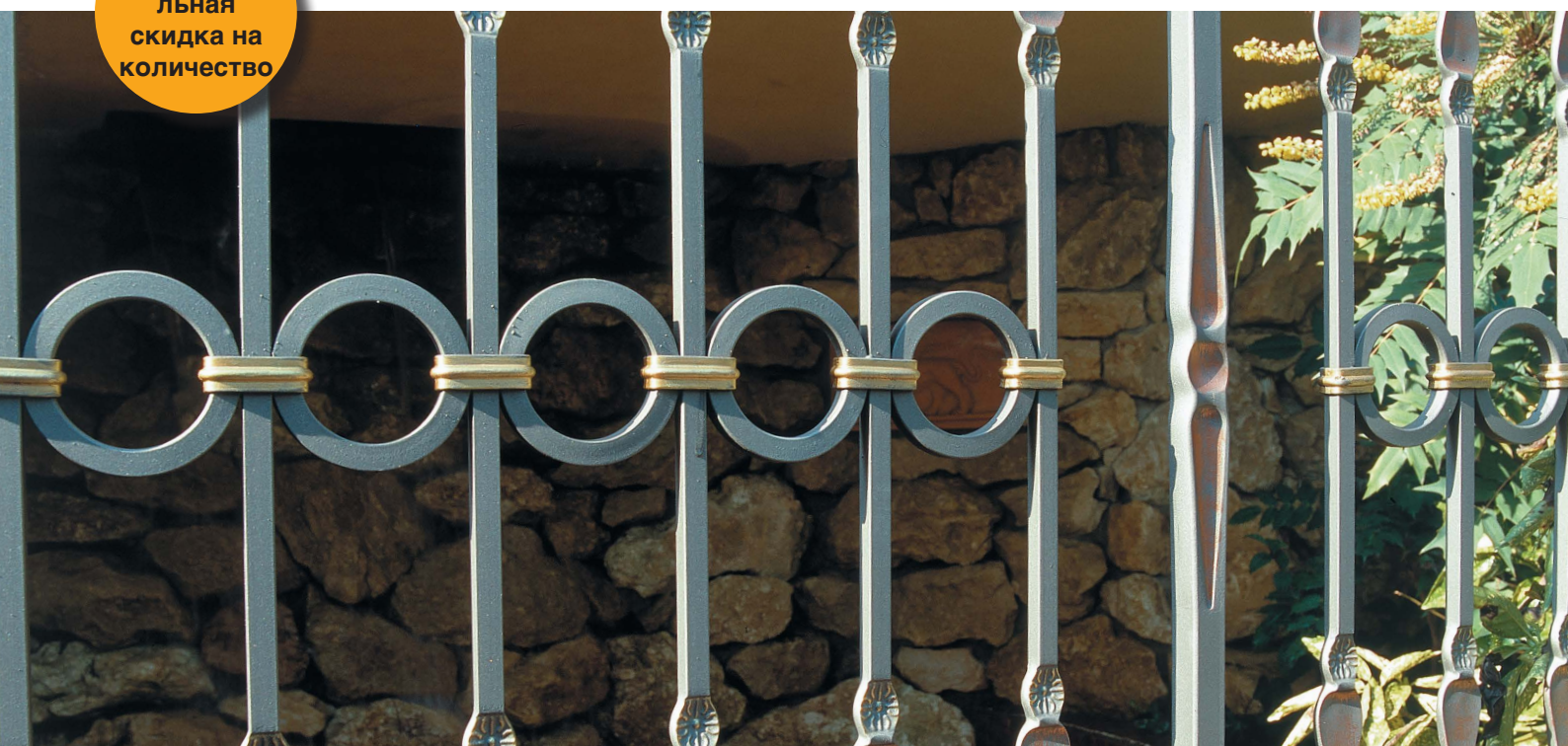
Art. 1320/17 ∅ 20 x 6 mm 115 x 190 mm
