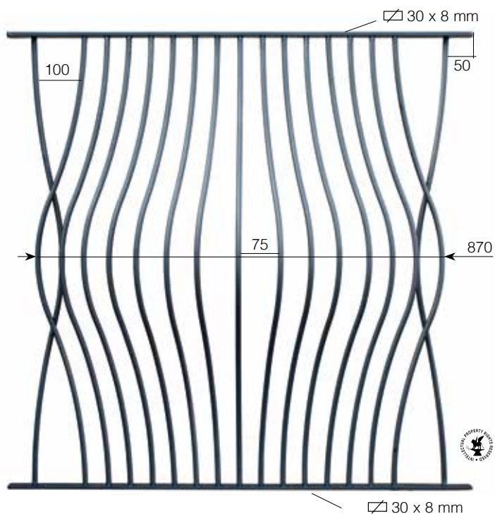
Арт. GD288/1 Ø 12 mm L1000 mm H 1000 mm
