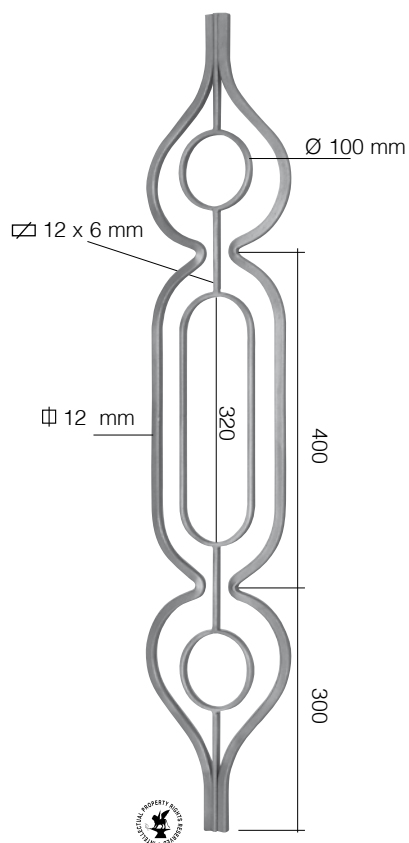
Арт. GD69/1 ∅ 12 mm L 210 mm H 1000 mm
