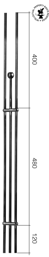
Арт. GD39/2 Ø 12 mm H 1000 mm L 60 mm
