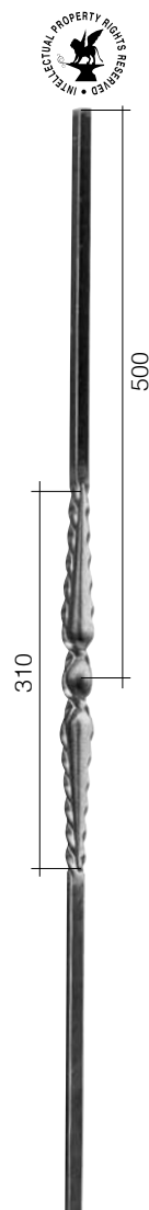
Арт. 1730/7 \Phi 12 x 12 mm L 25 mm H 1000 mm
