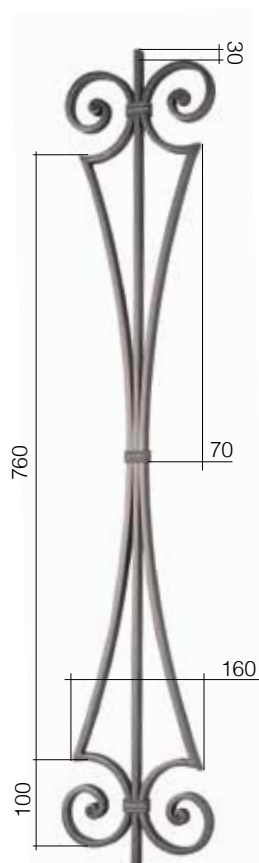
Арт. GD280/1 ∅ 14 x 8 mm L 200 mm H 1000 mm
