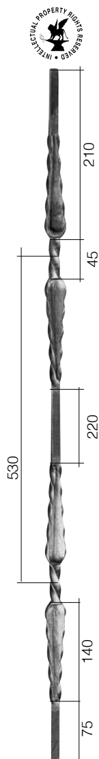
Арт. 1730/1 \Phi 12 x 12 mm L 25 mm H 1000 mm
