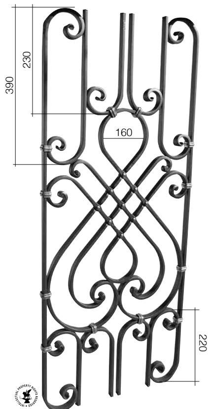
Арт. GD99/1 □ 16 x 8 mm L 420 mm H 1000 mm
