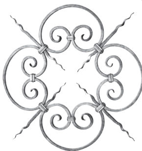
Art. 1012/2 12 x 12 mm Ø 730 mm
