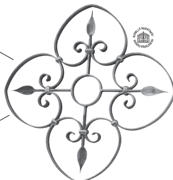
Art. 1649/1 ▧ 20 x 6 mm Ø 560 mm
