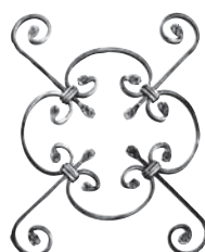
Art. 18/B/1 12 x 6 mm H 350 mm L 270 mm
