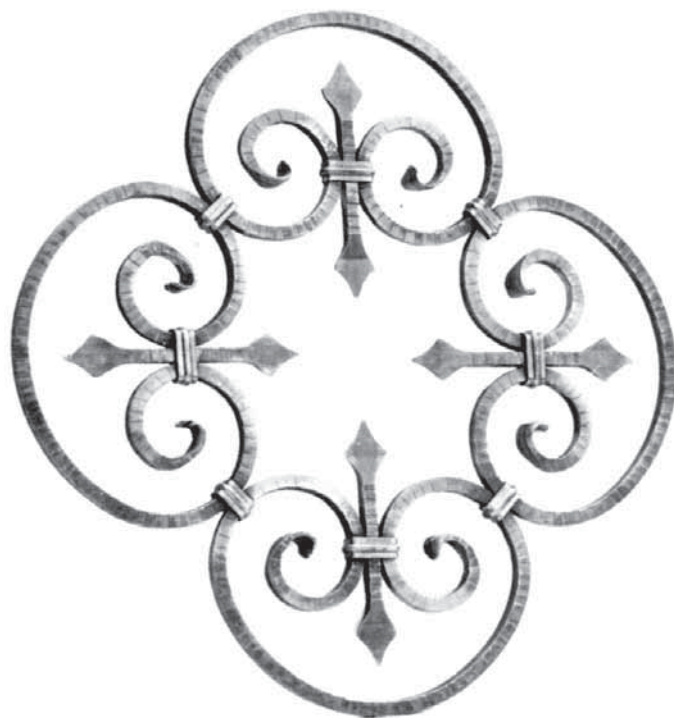
Art. 24/3 \square 12 x 12 mm \varnothing 600 mm
