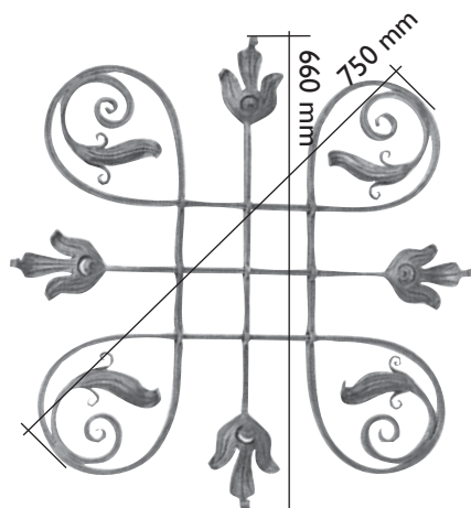
Art. 680/2 \nabla 16 x 8 mm 590 x 590 mm
